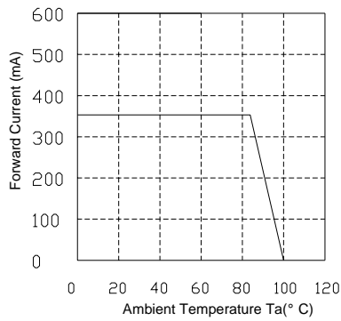
Derating
